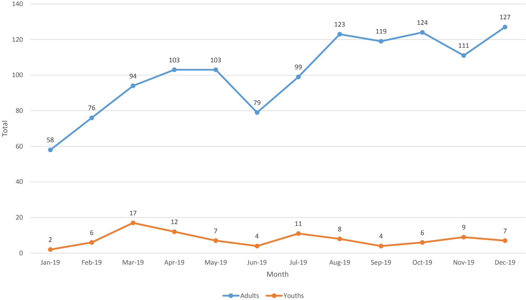
Telford Custody - Use of Force (Prior to Custody) - Adults and Youths - 2019
